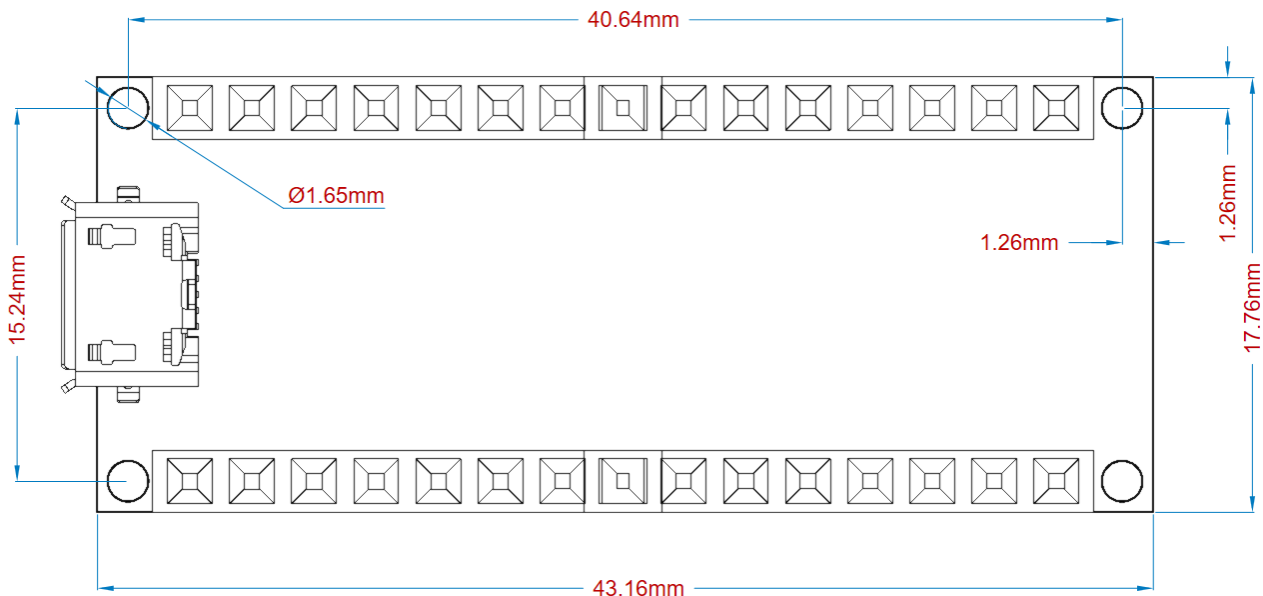
Board layout
