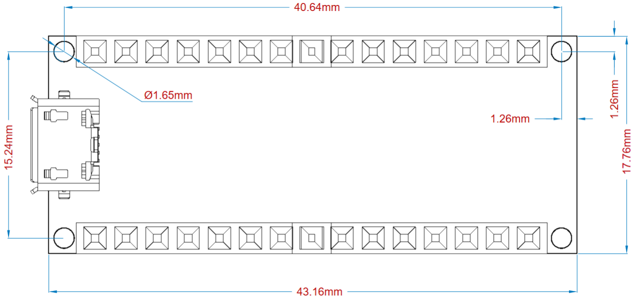
Board layout
