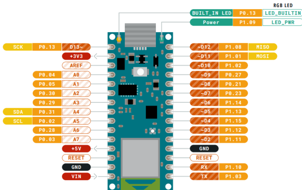
Pinout
