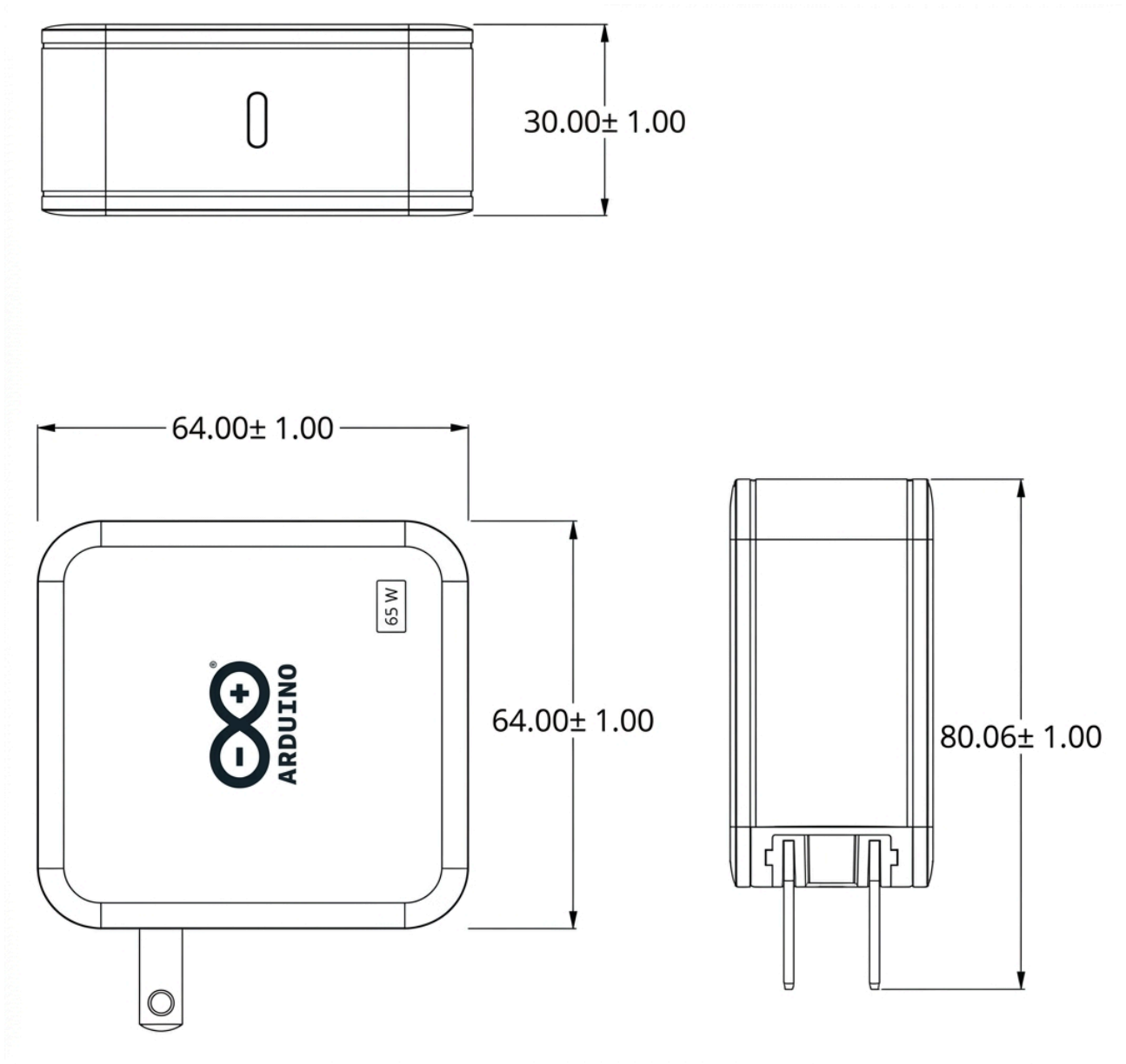
Power Supply Dimensions
