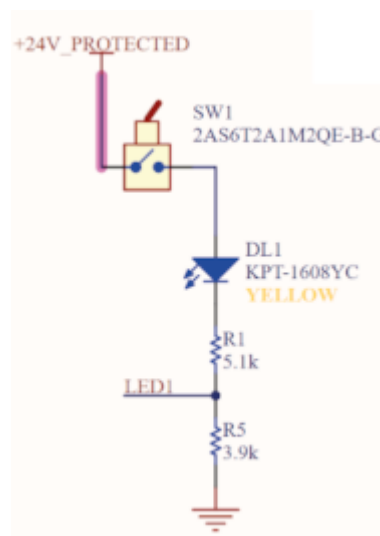
toggle switch scheme
