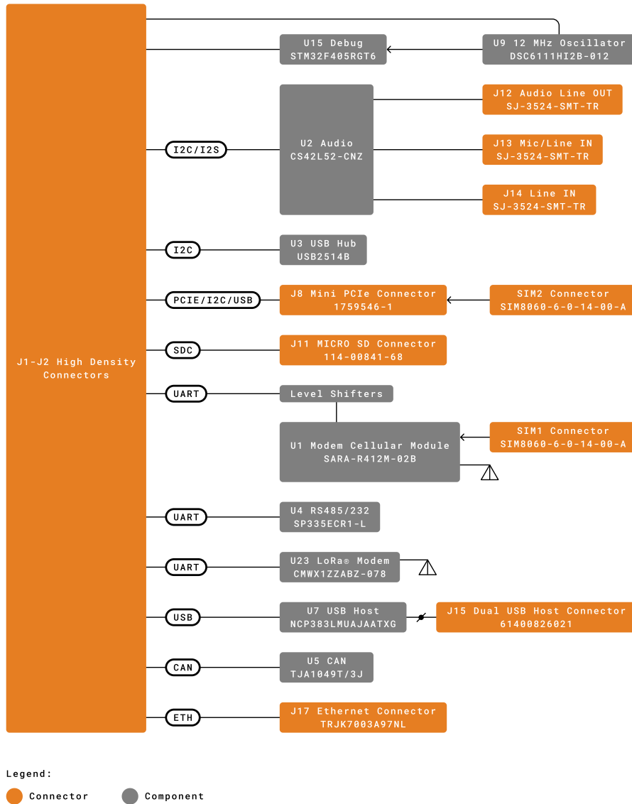
Block Diagram
